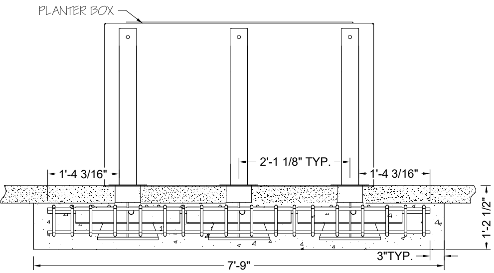
2 FRONT VIEW PL-40-003-1 Scale: None
