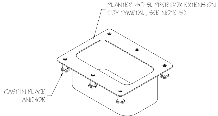
3 ISOMETRIC VIEW OF SLIPPER BOX EXT. PL-40-003-2 Scale: None
