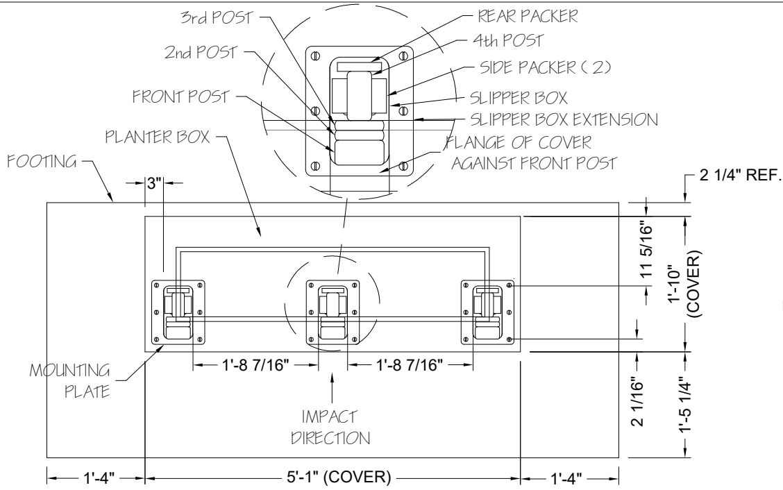
1 PLAN VIEW PL-40-003-1 Scale: None
