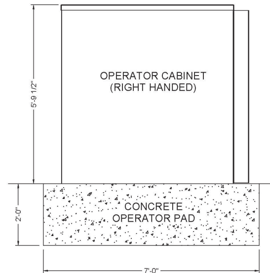
ELEVATION VIEW
