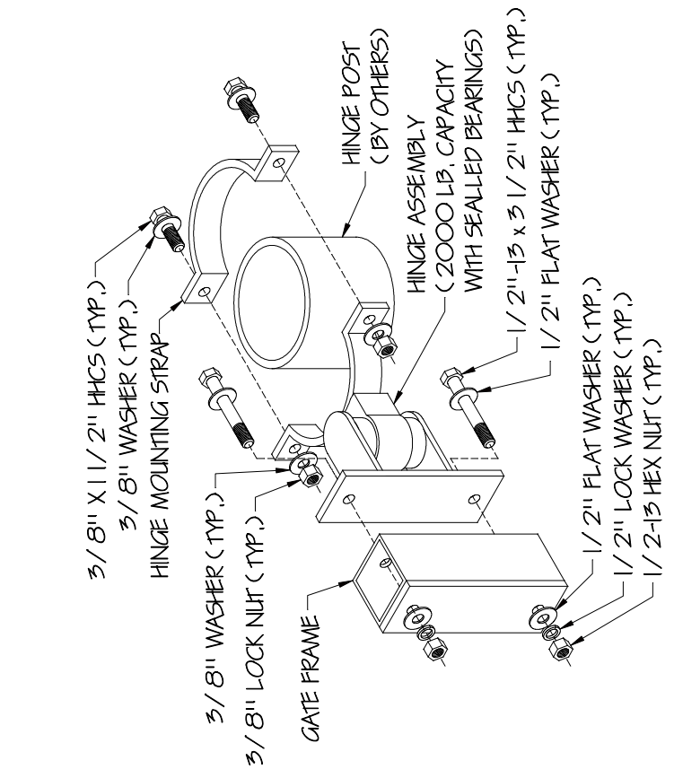
2 HINGE ASSEMBLY SW104-2 Scale: None
